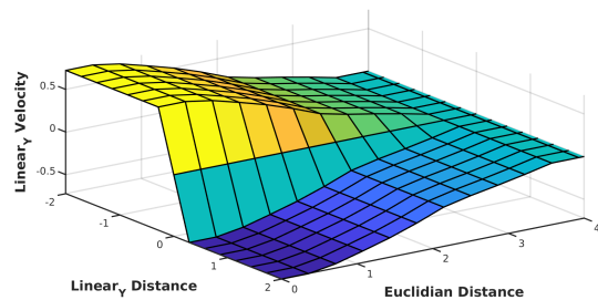
FIGURE 5. Lead drone avoid obstacles control system - Velocity maps generated by fuzzy position control system. (A) Obstacle detection and measured distances to the drone. (B) Map of the linear velocity in the Z-axis, about the linear error (Euclidean distance) and linear error in Z-axis (Z-axis difference) between the drone position and obstacle detected. (C) Map of the linear velocity in the Y-axis, about the linear error (Euclidean distance) and linear error in Y-axis (Y-axis difference) between the drone position and obstacle detected.
