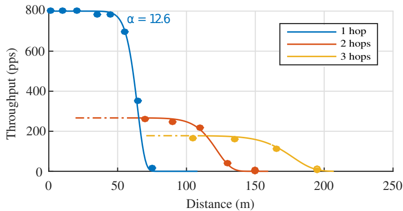
Figure 3.6: Measured throughput at different end-to-end network lengths, using distinct number of hops. Inside their slots, nodes transmit 200-byte packets at a rate of B \approx 800\text{ pkts/s} . UAVs are all oriented parallel to each other.
