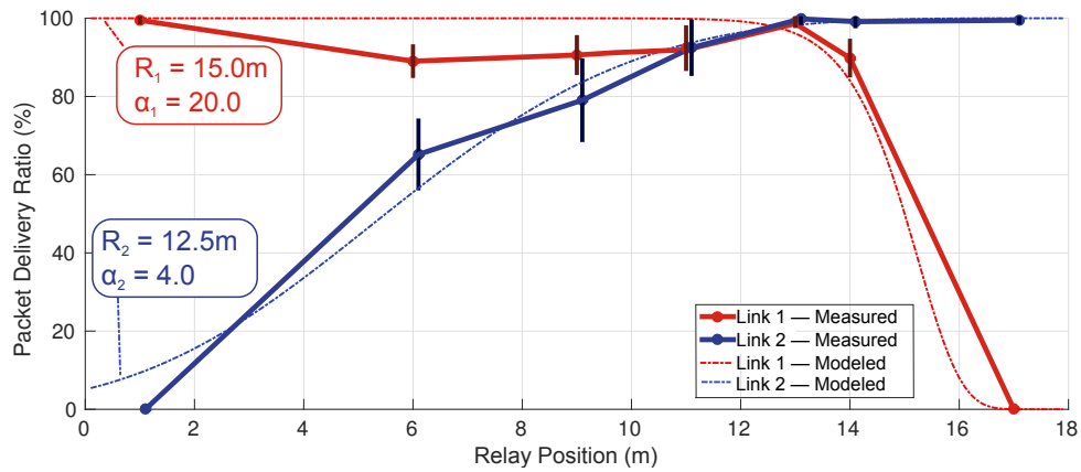
Figure 6.10: Experimentally measured packet delivery ratio at the first (red) and second (blue) links, with respective standard deviation, at different static relay positions. Best scenario when relay is closer to sink ( x = 13\text{m} ) leading to end-to-end PDR \approx 100\% . Dashed lines are superimposed regressions of Equation 6.1 on experimental data.
