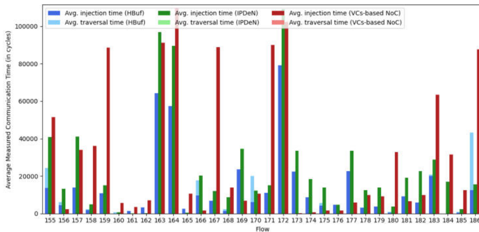
Fig. 45. Average measured communication time (Orion test case) 5-5
