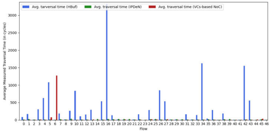
Fig. 27. Average measured traversal time (Orion test case) 1-5
