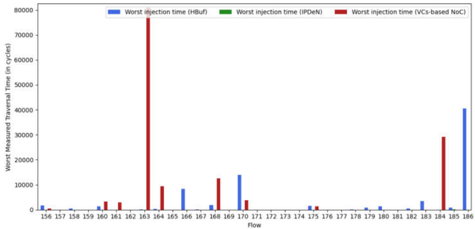
Fig. 15. Worst measured traversal time (Orion test case) 5-5
