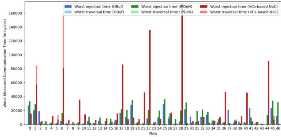
Fig. 17. Worst measured communication time (Orion test case) 1-5
