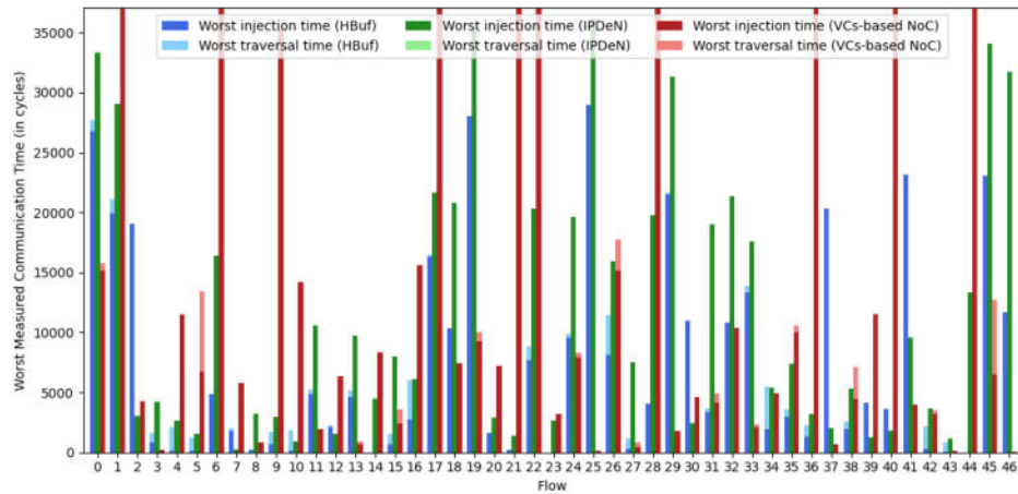
Fig. 18. Worst measured communication time (Zoom) (Orion test case) 1-5
