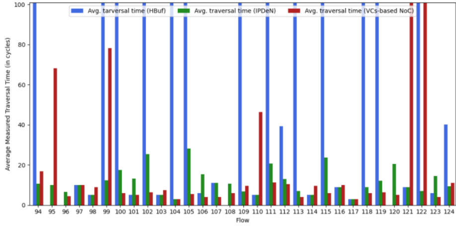
Fig. 32. Average measured traversal time (Zoom) (Orion test case) 3-5
