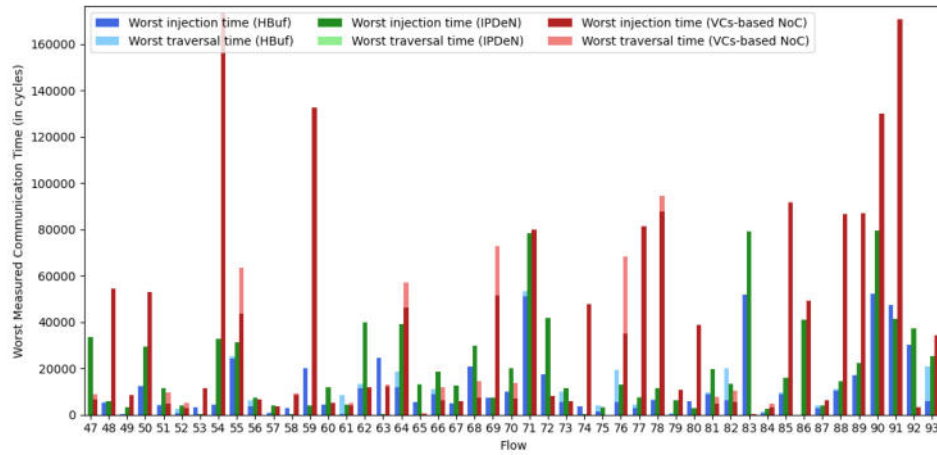
Fig. 19. Worst measured communication time (Orion test case) 2-5
