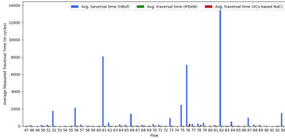
Fig. 29. Average measured traversal time (Orion test case) 2-5
