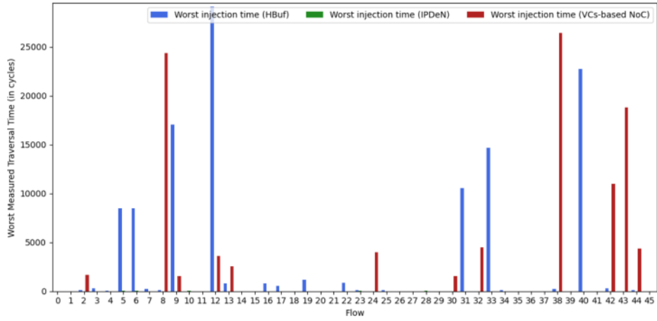
Fig. 1. Worst measured traversal time (Synthetic test case)
