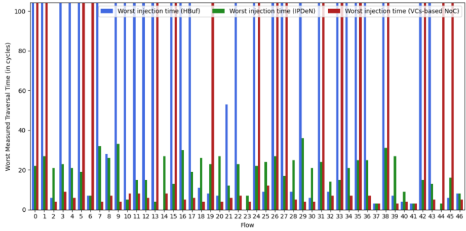
Fig. 8. Worst measured traversal time (Zoom) (Orion test case) 1-5
