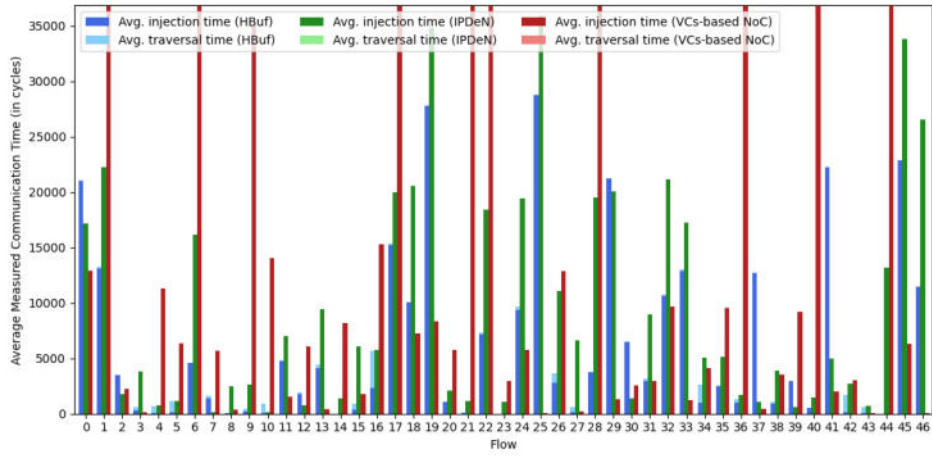
Fig. 38. Average measured communication time (Zoom) (Orion test case) 1-5
