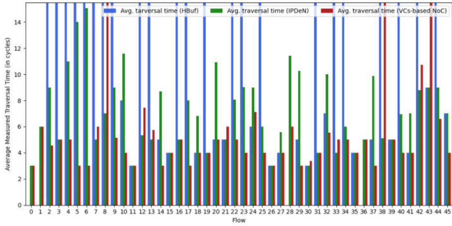
Fig. 5. Average measured traversal time (Zoom) (Synthetic test case)
