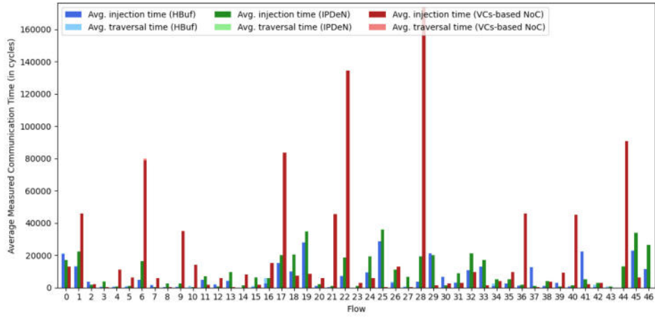
Fig. 37. Average measured communication time (Orion test case) 1-5
