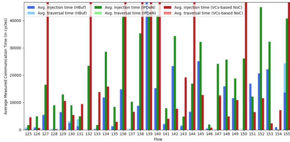
Fig. 44. Average measured communication time (Zoom) (Orion test case) 4-5
