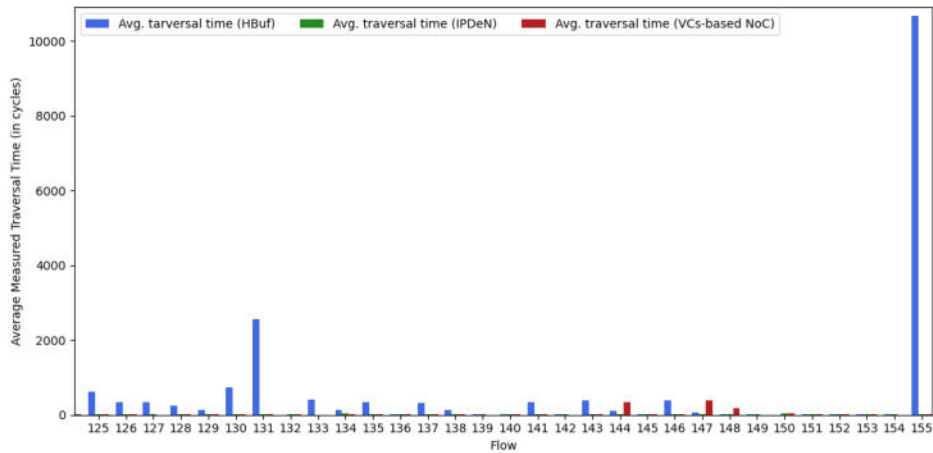
Fig. 33. Average measured traversal time (Orion test case) 4-5
