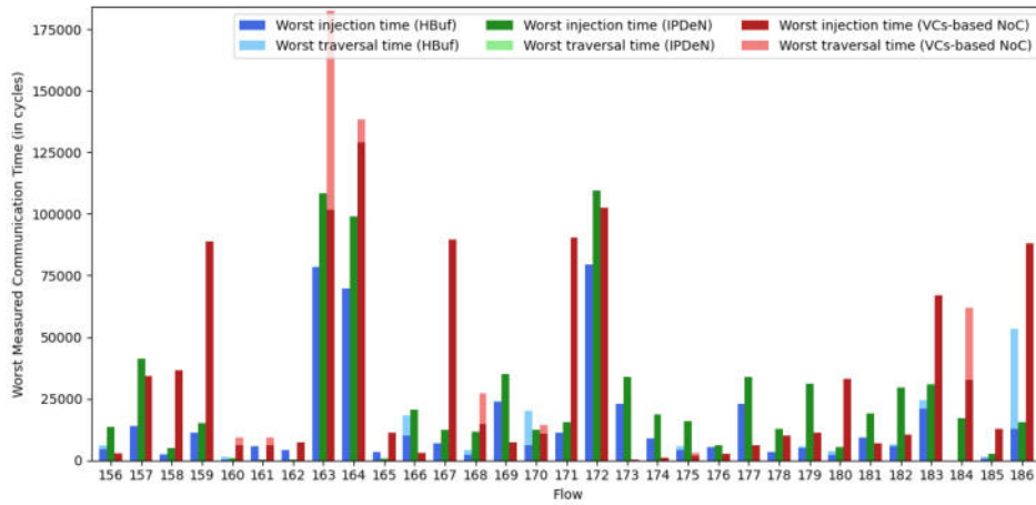
Fig. 25. Worst measured communication time (Orion test case) 5-5
