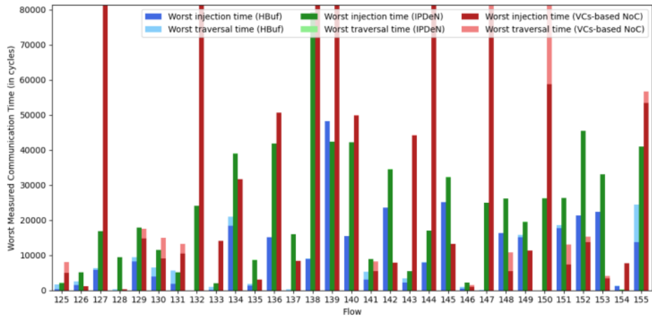
Fig. 24. Worst measured communication time (Zoom) (Orion test case) 4-5
