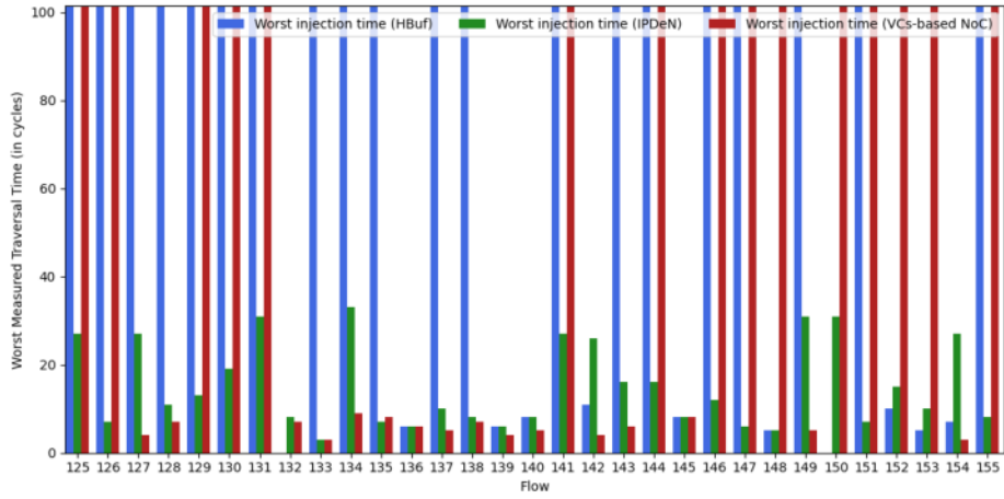
Fig. 14. Worst measured traversal time (Zoom) (Orion test case) 4-5
