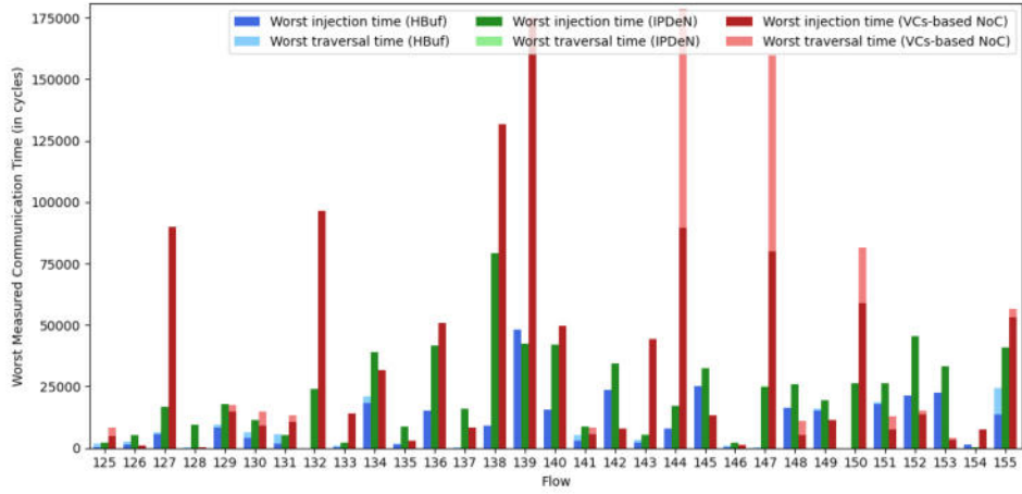
Fig. 23. Worst measured communication time (Orion test case) 4-5
