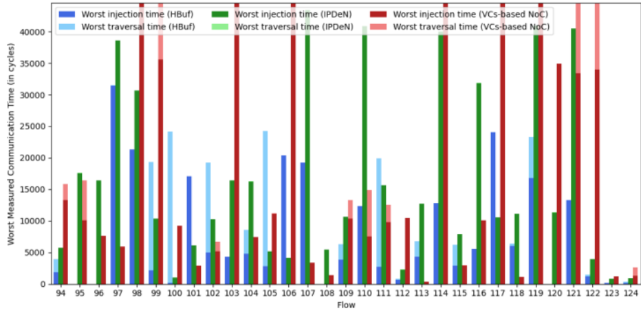
Fig. 22. Worst measured communication time (Zoom) (Orion test case) 3-5
