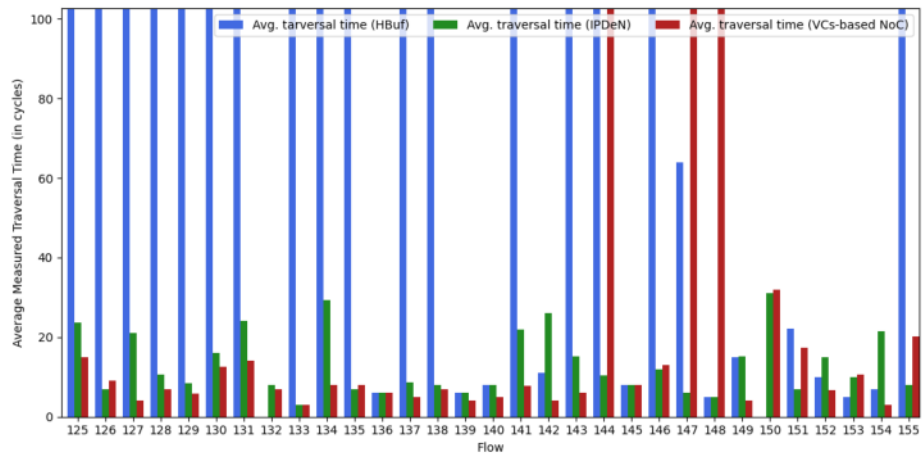
Fig. 34. Average measured traversal time (Zoom) (Orion test case) 4-5
