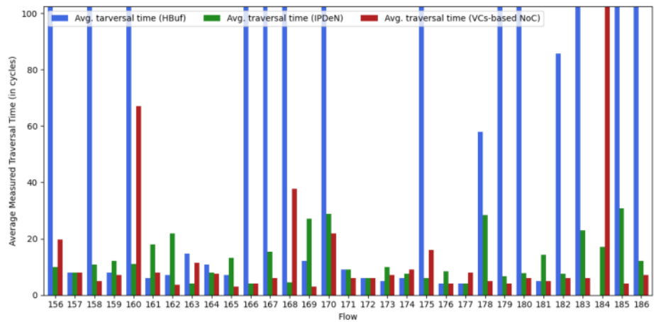
Fig. 36. Average measured traversal time (Zoom) (Orion test case) 5-5
