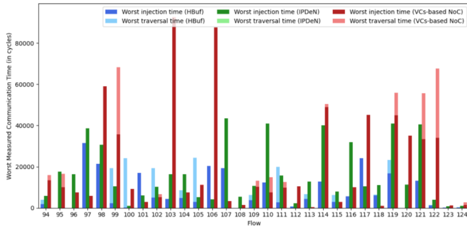
Fig. 21. Worst measured communication time (Orion test case) 3-5
