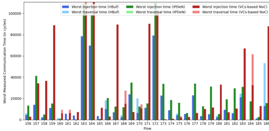
Fig. 26. Worst measured communication time (Zoom) (Orion test case) 5-5
