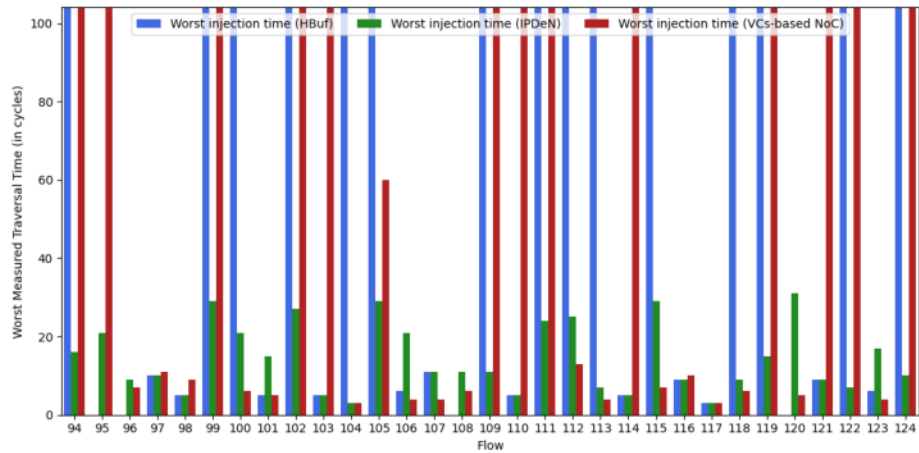
Fig. 12. Worst measured traversal time (Zoom) (Orion test case) 3-5
