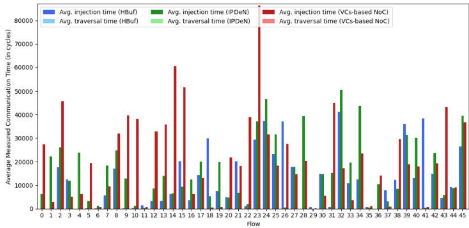
Fig. 6. Average measured communication time (Synthetic test case)
