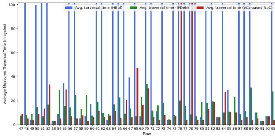
Fig. 30. Average measured traversal time (Zoom) (Orion test case) 2-5
