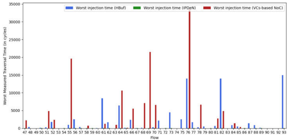
Fig. 9. Worst measured traversal time (Orion test case) 2-5
