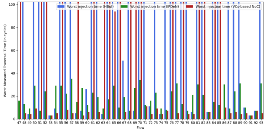
Fig. 10. Worst measured traversal time (Zoom) (Orion test case) 2-5
