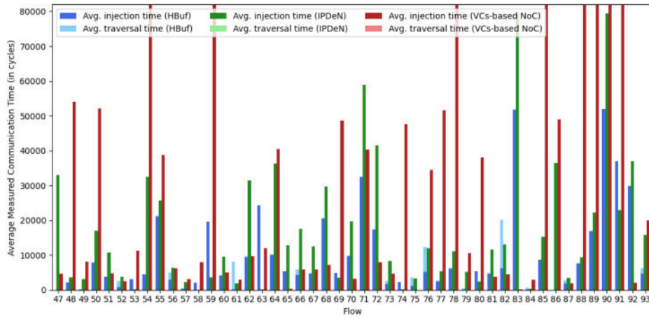
Fig. 40. Average measured communication time (Zoom) (Orion test case) 2-5
