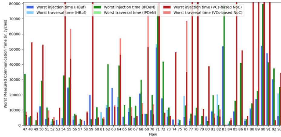
Fig. 20. Worst measured communication time (Zoom) (Orion test case) 2-5
