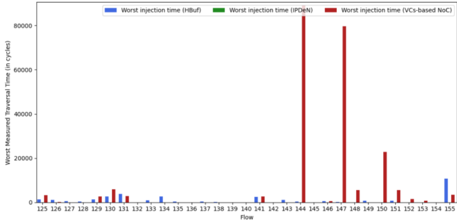
Fig. 13. Worst measured traversal time (Orion test case) 4-5
