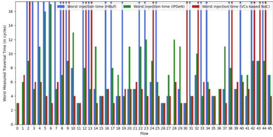
Fig. 2. Worst measured traversal time (Zoom) (Synthetic test case)
