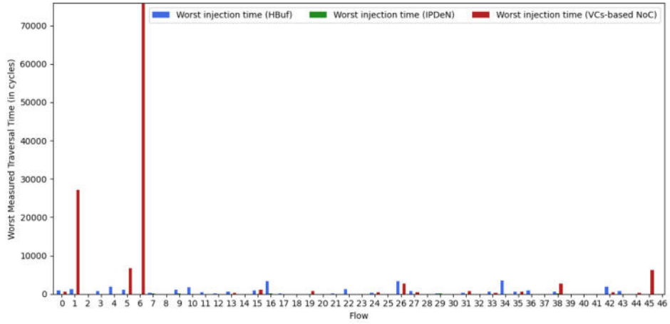
Fig. 7. Worst measured traversal time (Orion test case) 1-5
