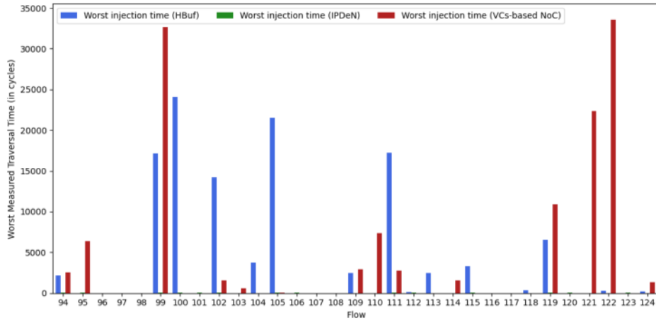
Fig. 11. Worst measured traversal time (Orion test case) 3-5
