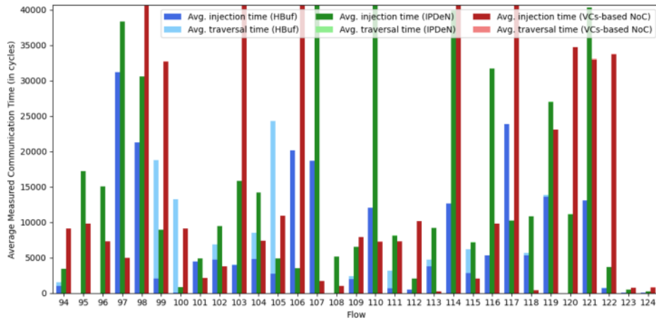
Fig. 42. Average measured communication time (Zoom) (Orion test case) 3-5
