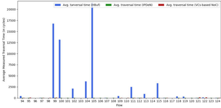
Fig. 31. Average measured traversal time (Orion test case) 3-5
