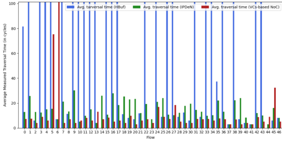
Fig. 28. Average measured traversal time (Zoom) (Orion test case) 1-5
