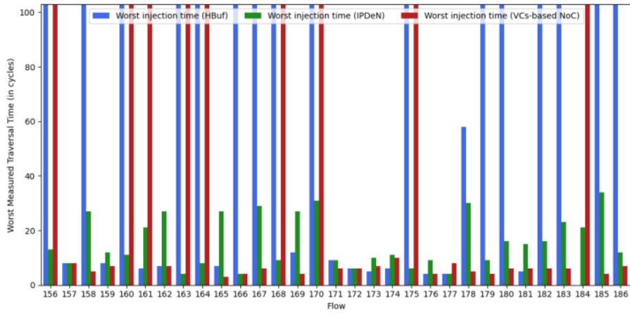
Fig. 16. Worst measured traversal time (Zoom) (Orion test case) 5-5
