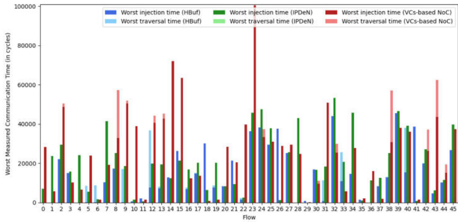
Fig. 3. Worst measured communication time (Synthetic test case)
