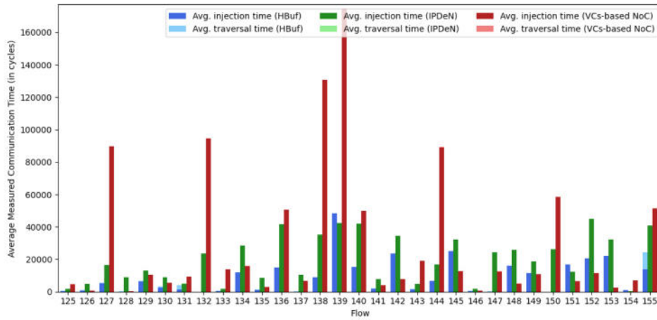
Fig. 43. Average measured communication time (Orion test case) 4-5
