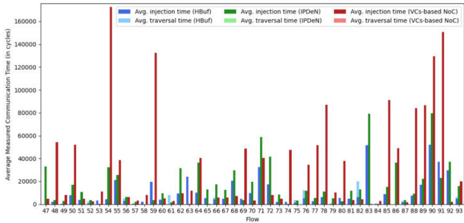
Fig. 39. Average measured communication time (Orion test case) 2-5
