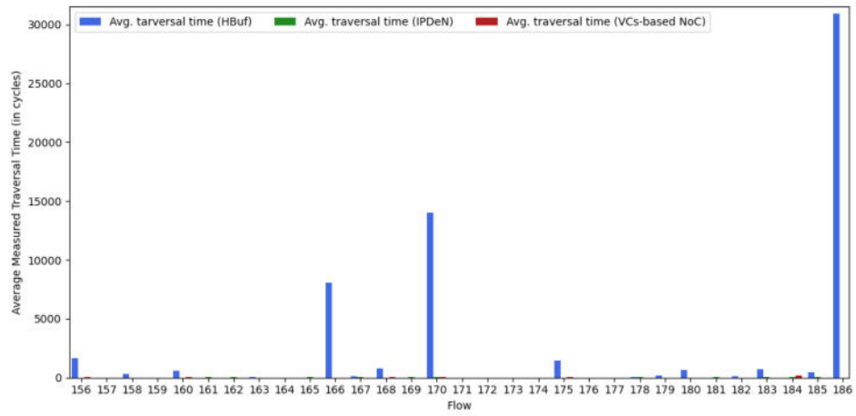
Fig. 35. Average measured traversal time (Orion test case) 5-5
