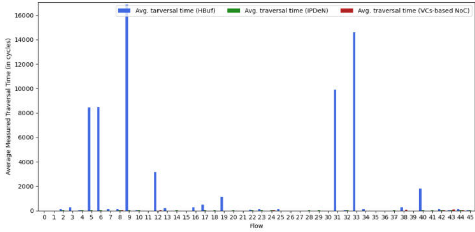
Fig. 4. Average measured traversal time (Synthetic test case)
