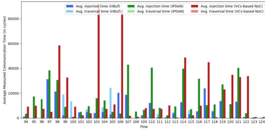
Fig. 41. Average measured communication time (Orion test case) 3-5
