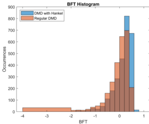
Fig. 6. Histograms of the BFTs of the Kernel predictor with raw-data and with a Block Hankel Matrix.
