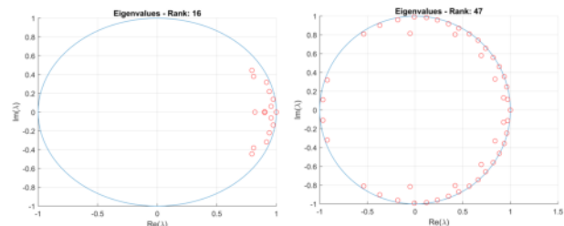
Fig. 5. The discrete-time eigenvalues estimated by the DMD with raw-data (LEFT) and using Hankel block matrix (RIGHT).
