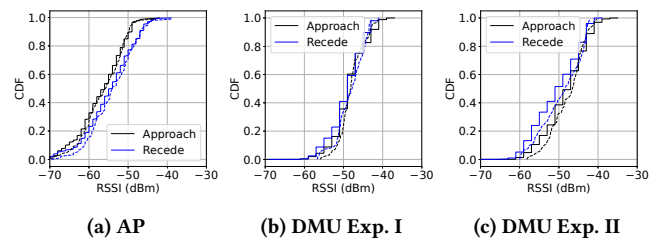
Figure 8: RSSI CDF of the raw (full line) and aggregated (dashed line) data for the three configurations.
