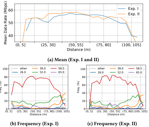
Figure 11: Negotiated data rates as a function of distance for experiments I and II. We consider a bin size of 5 m.
