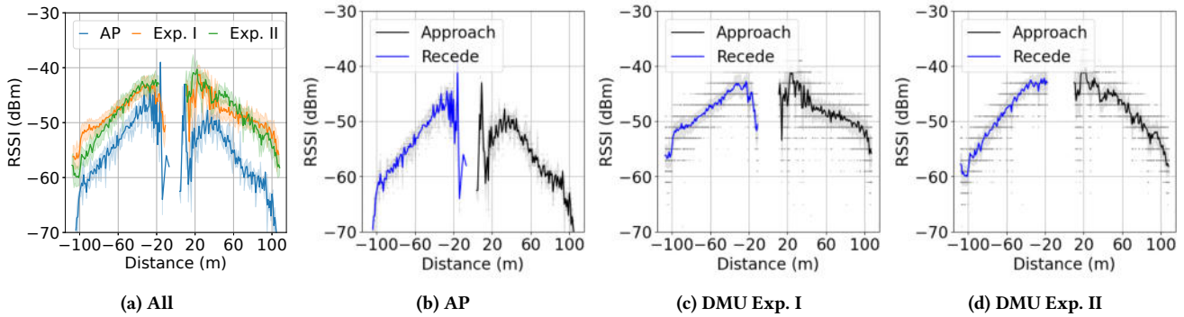
Figure 7: RSSI for approach and recede travel directions. Each tendency line [shaded area] in (a), (b), (c) and (d) is the mean RSSI [standard deviation above/below the mean RSSI] for the given distance bin and travel direction. The points in (b), (c) and (d) represent raw RSSI measurements for each configuration.
