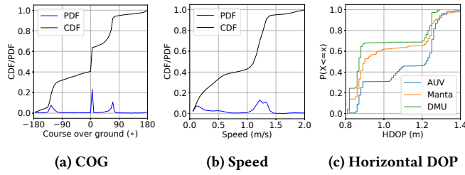
Figure 4: Mobility data analysis, namely Course of Ground (COG), Speed and Horizontal Dilution of Precision (HDOP).
