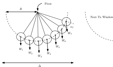
Fig. 13: Pendulum task model
